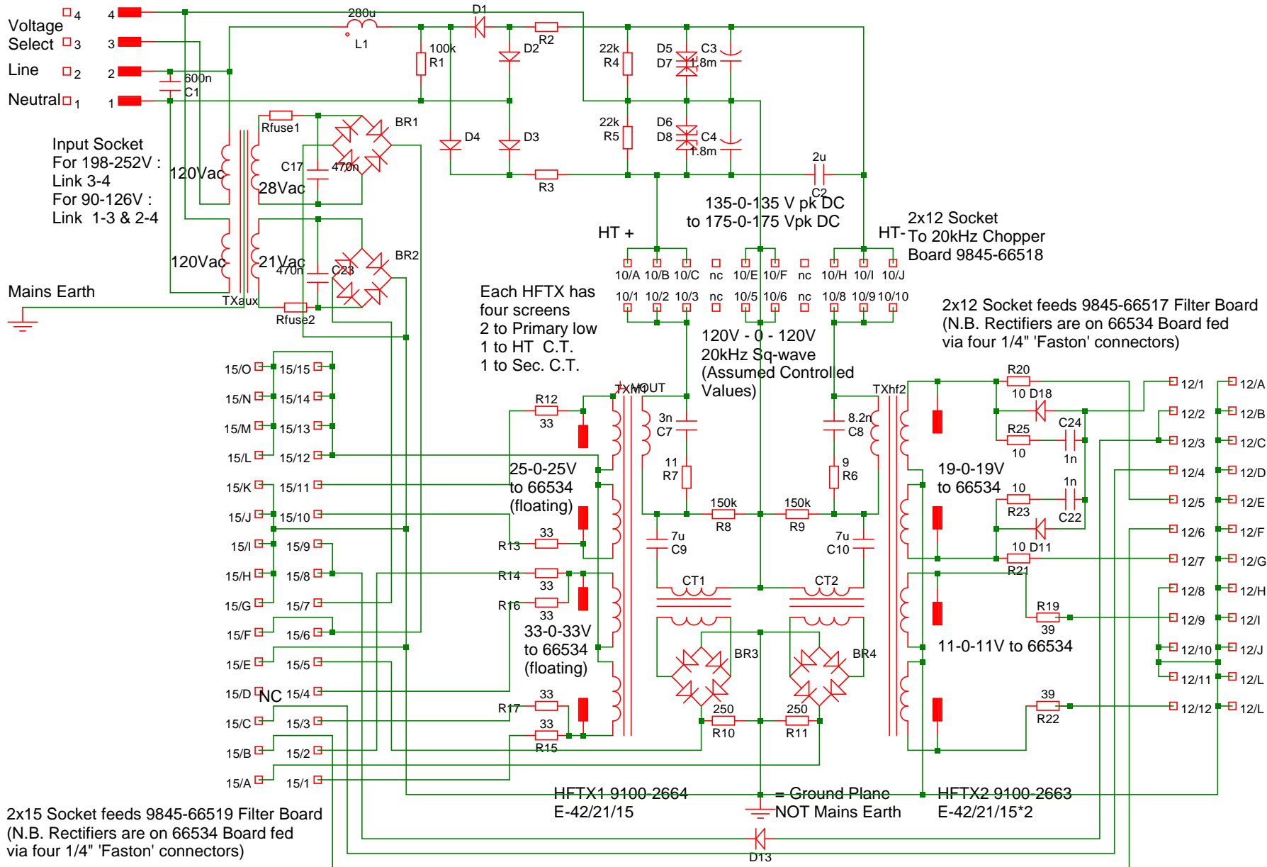
HP 9845-66520 Input Power Board
