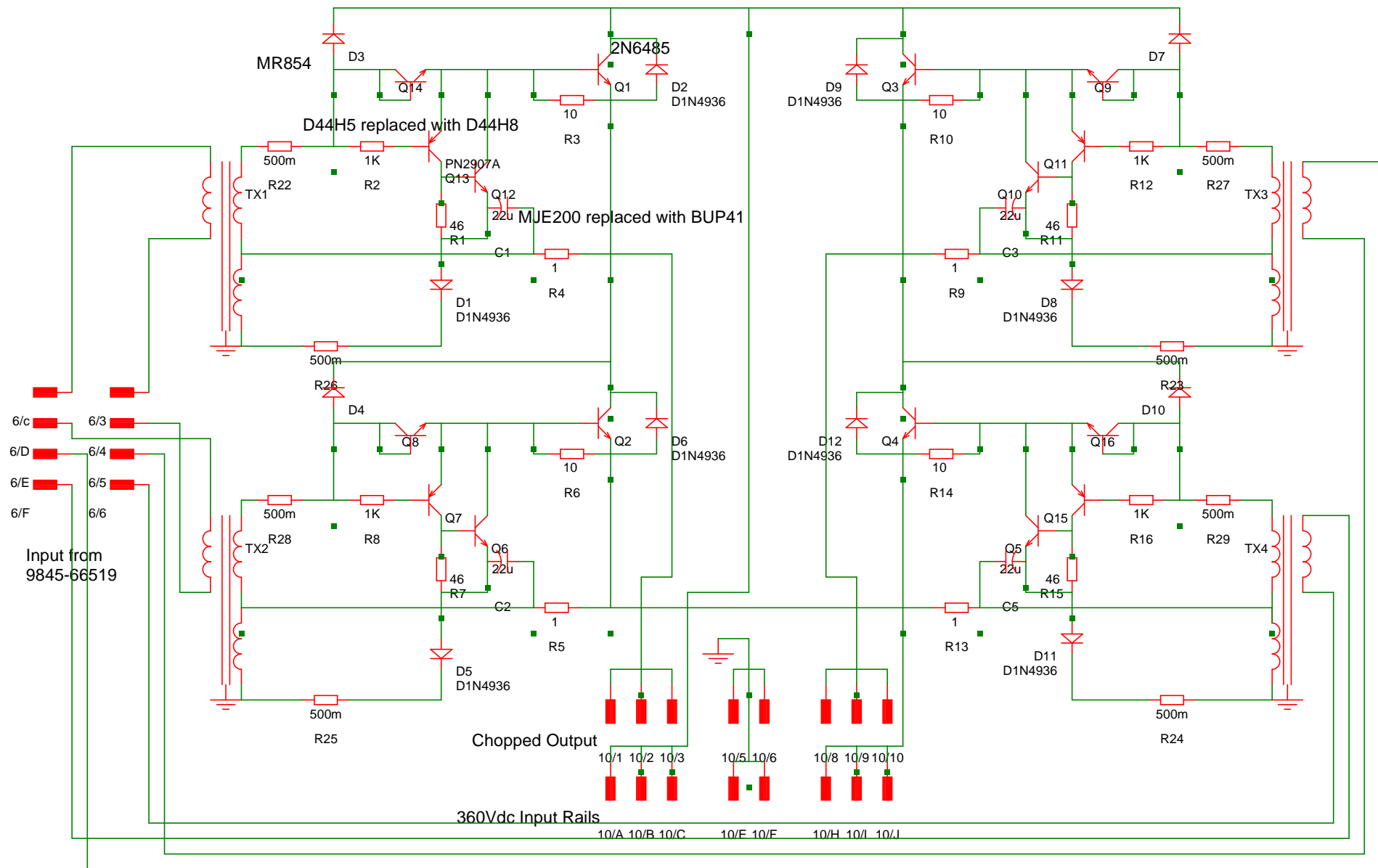
HP 9845-66518 PSU Input Bridge Chopper Circuit
