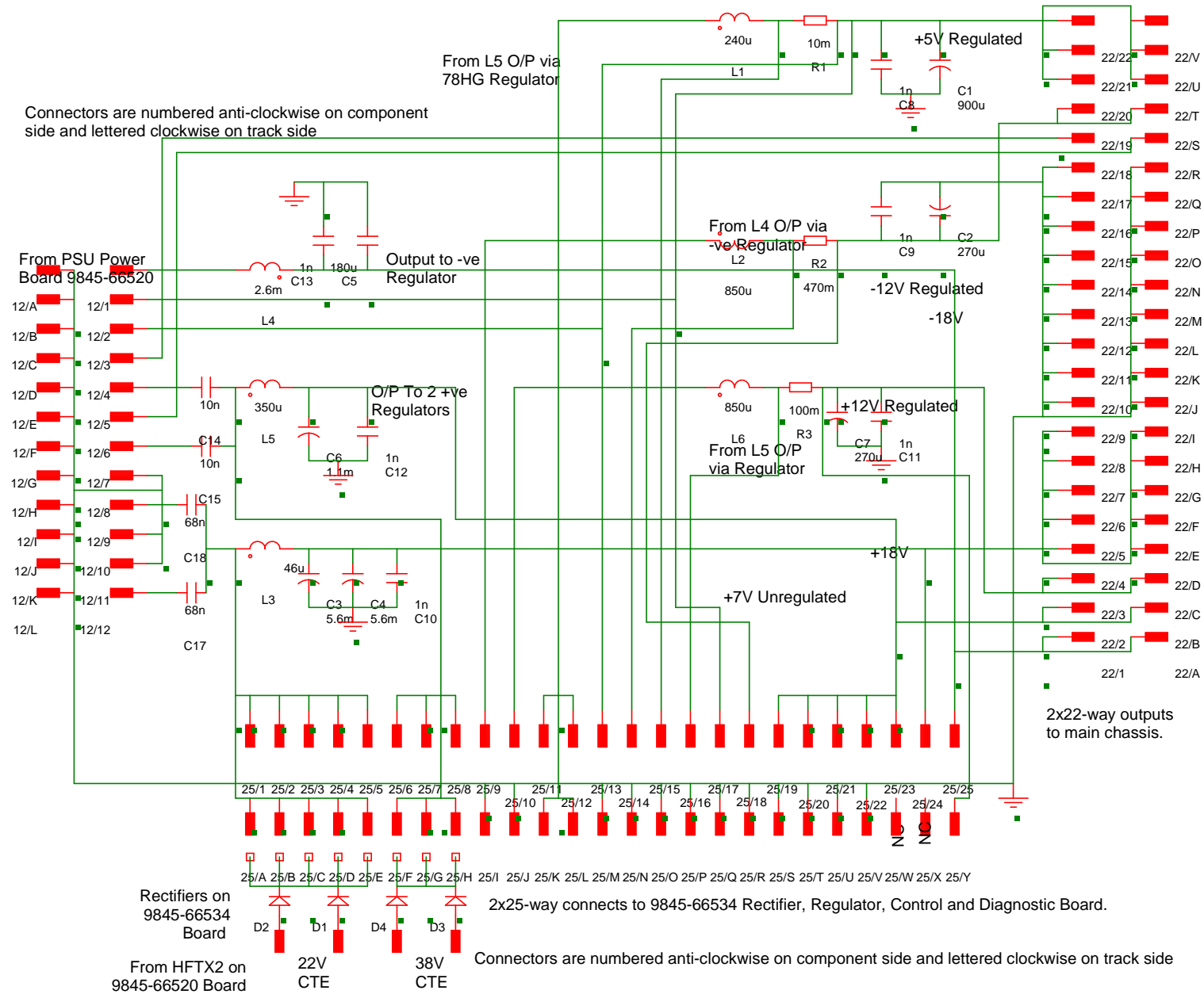
HP 9845-66517 PSU Filter Board
